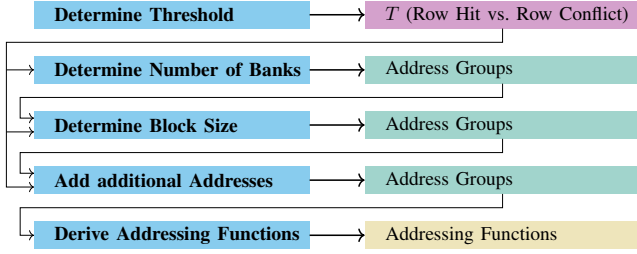
Figure 1. Overview of the reverse-engineering process. Actions (shown on the left side) lead to results (shown on the right side) and require some of the results of previous actions. Different results are depicted in different colors. Actions that require and return address groups add more addresses to the existing groups.
